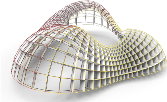
Fig. 4. Meshes are F-transforms if they share a support structure. Their respective face images are parallel meshes. Here three F-transforms (shown by yellow, red, and black edges) have been created by simply parallel translating the face image M_F of a base mesh M .
