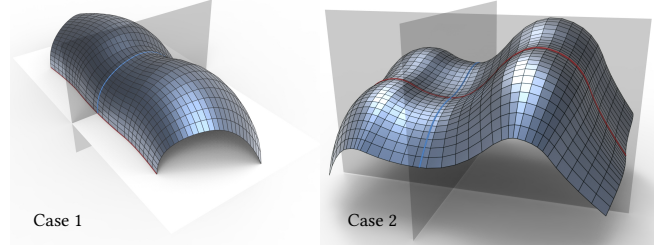
Fig. 17. Examples of conical PP meshes designed via their principal planar sections, using the explicit representations derived in §4.1.1 and §4.1.2.
