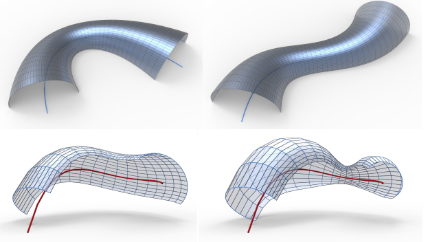
Fig. 18. Design of conical P meshes via the channel surface approach of § 4.2.3. Here we show Steps 2+3 of the construction. In the top row the radius function is the same for both examples shown, but the spine curve is different. In the bottom row the reverse is true.
