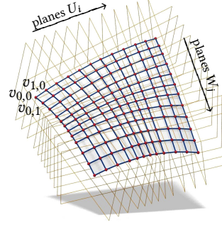
Fig. 7. Theoretical construction of a PP mesh from Cauchy initial data, if planes U_0, U_1, \dots and W_0, W_1, \dots are given. The vertex v_{i+1,j+1} is found from v_{i,j}, v_{i,j+1}, v_{i+1,j} by intersecting the plane spanned by these three vertices with the straight line U_{i+1} \cap W_{j+1} .
